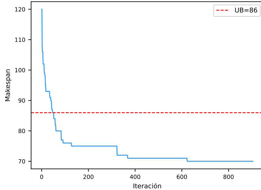
Brandimarte — Mk06
